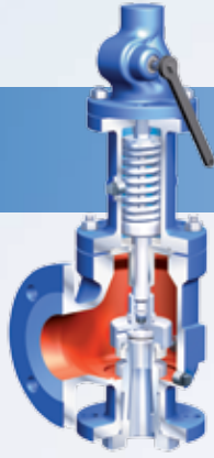
Full Nozzle Safety valve (API 526) ARI-REYCO™
