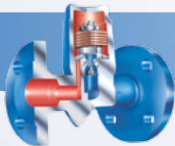
Steam traps CONA® (mechanical ball float / thermostatic / bimetallic and membrane / thermodynamic)
