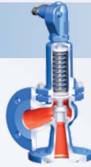
Proportional Lift Safety valve (DIN) SAFE P
