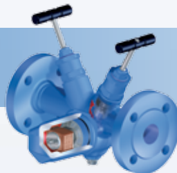
Steam trap with multi-valving technology (incl. stop valve, strainer, check valve, drain valve)
