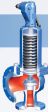
High Lift Safety valve (ASME & DIN) SAFE
