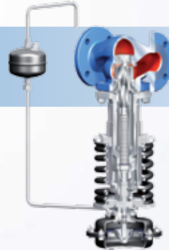
Excess pressure valve PREDEX®
